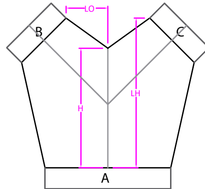
Reducing Y Branch
